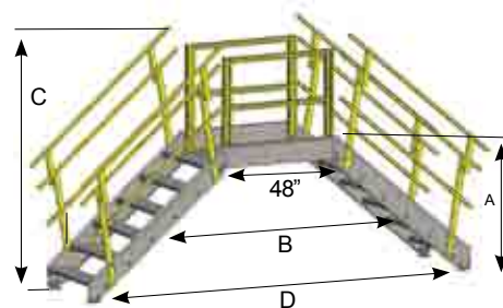
Stair Crossover Bridge
